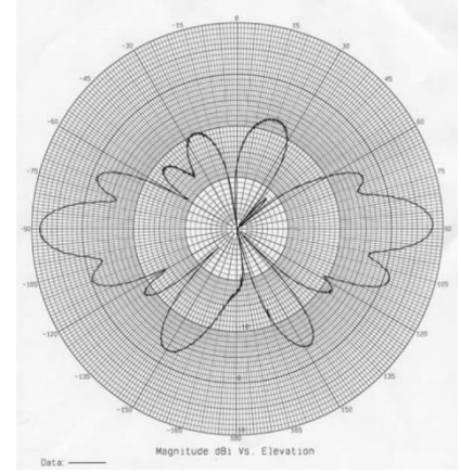
ECO8-2400 Series – Elevation Plot
