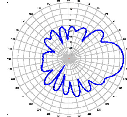
2500 MHz Azimuth
