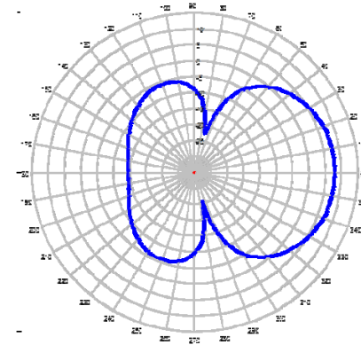
460 MHz Azimuth
